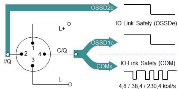
Fig. 6: Port interface extension
