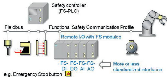
Fig. 1: FS communication
