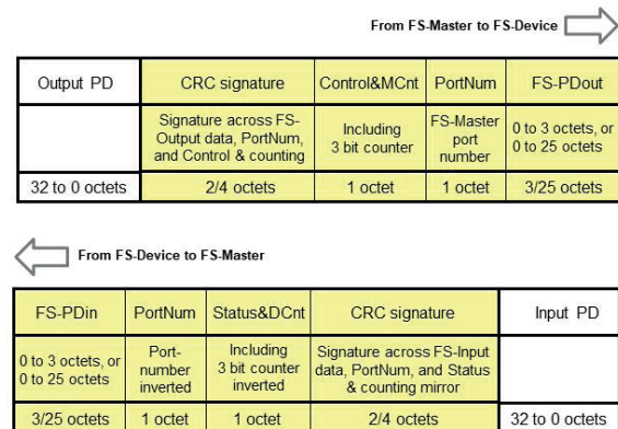
Fig. 7: Messages with Safety PDU
