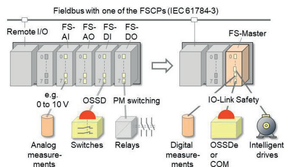
Fig. 2: Remote I/O
