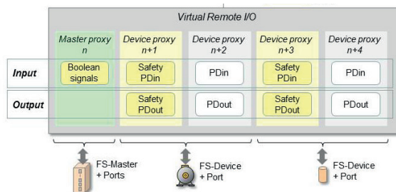
Fig. 12: Role model for mapping
