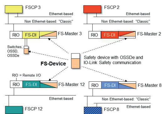
Fig. 4: Single platform solution
