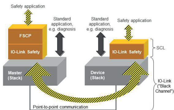
Fig. 5: “Black Channel” principle
