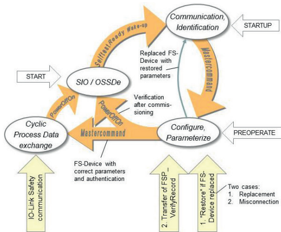
Fig. 9: Start-up of FS-Device
