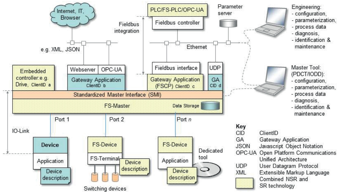
Fig. 11: Positioning of IO-Link Safety
